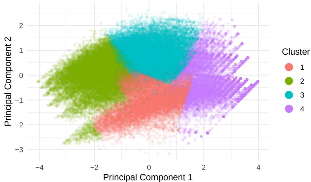
K-Means Clusters Visualized via PCA (k=4)
